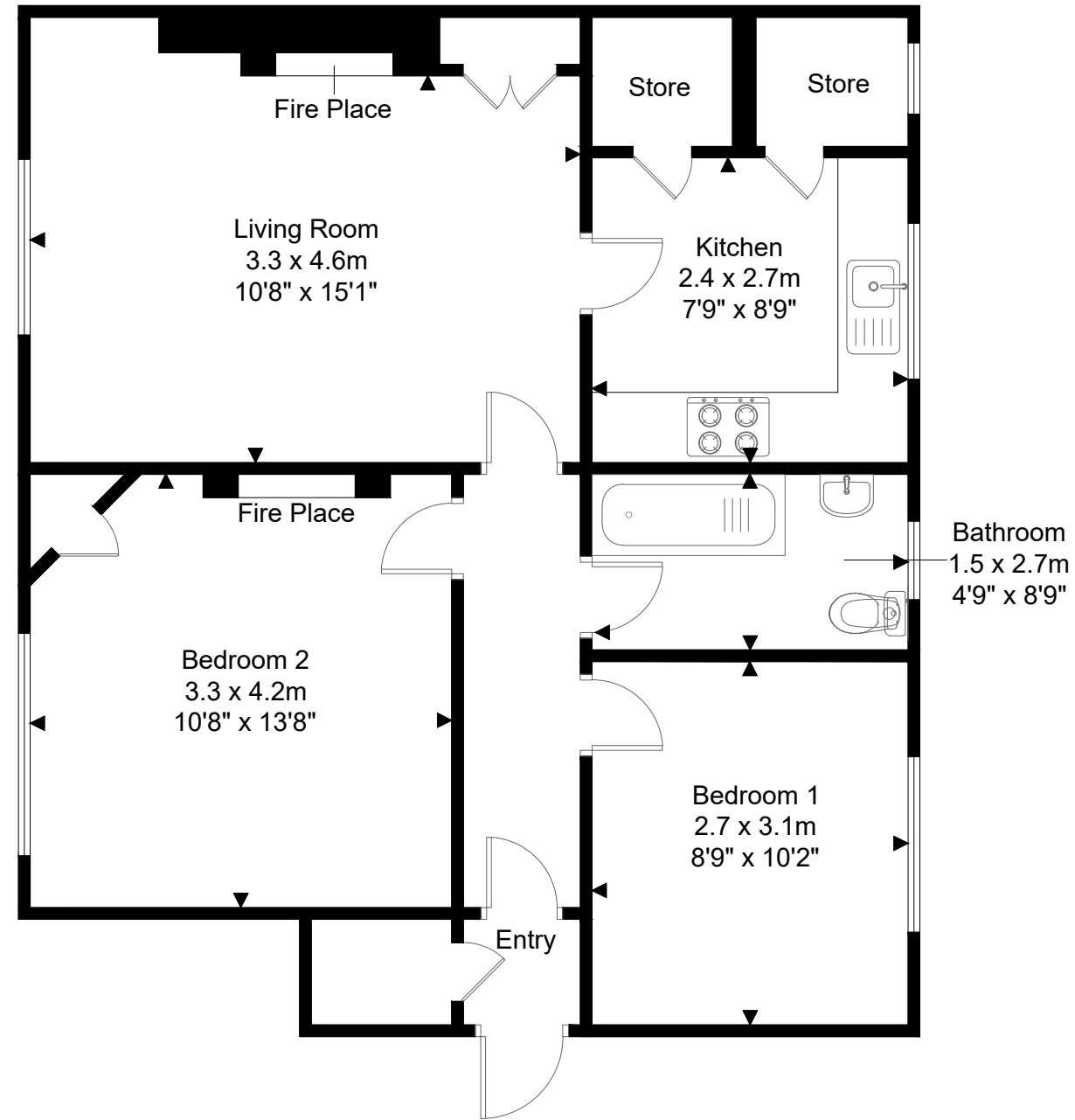
Ground Floor
